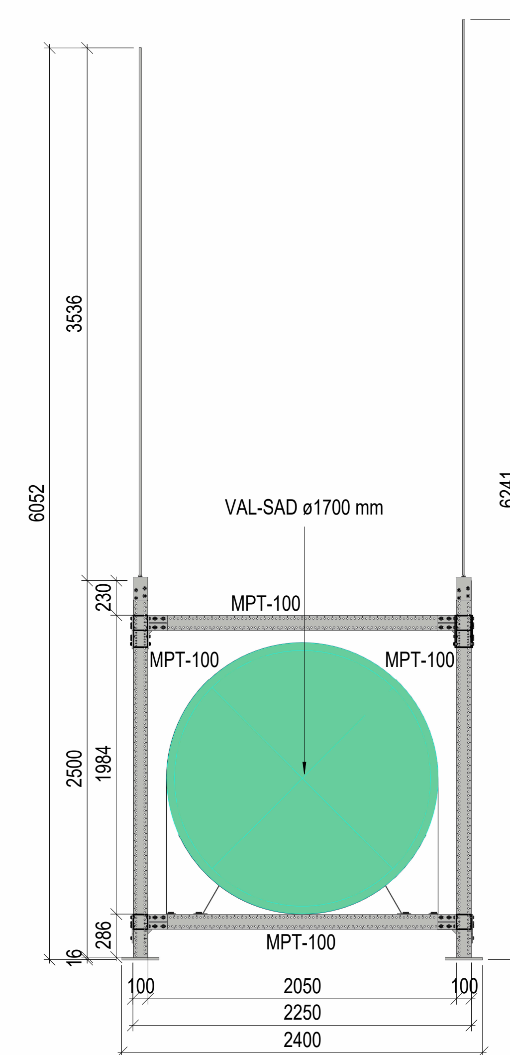
SECTION C
