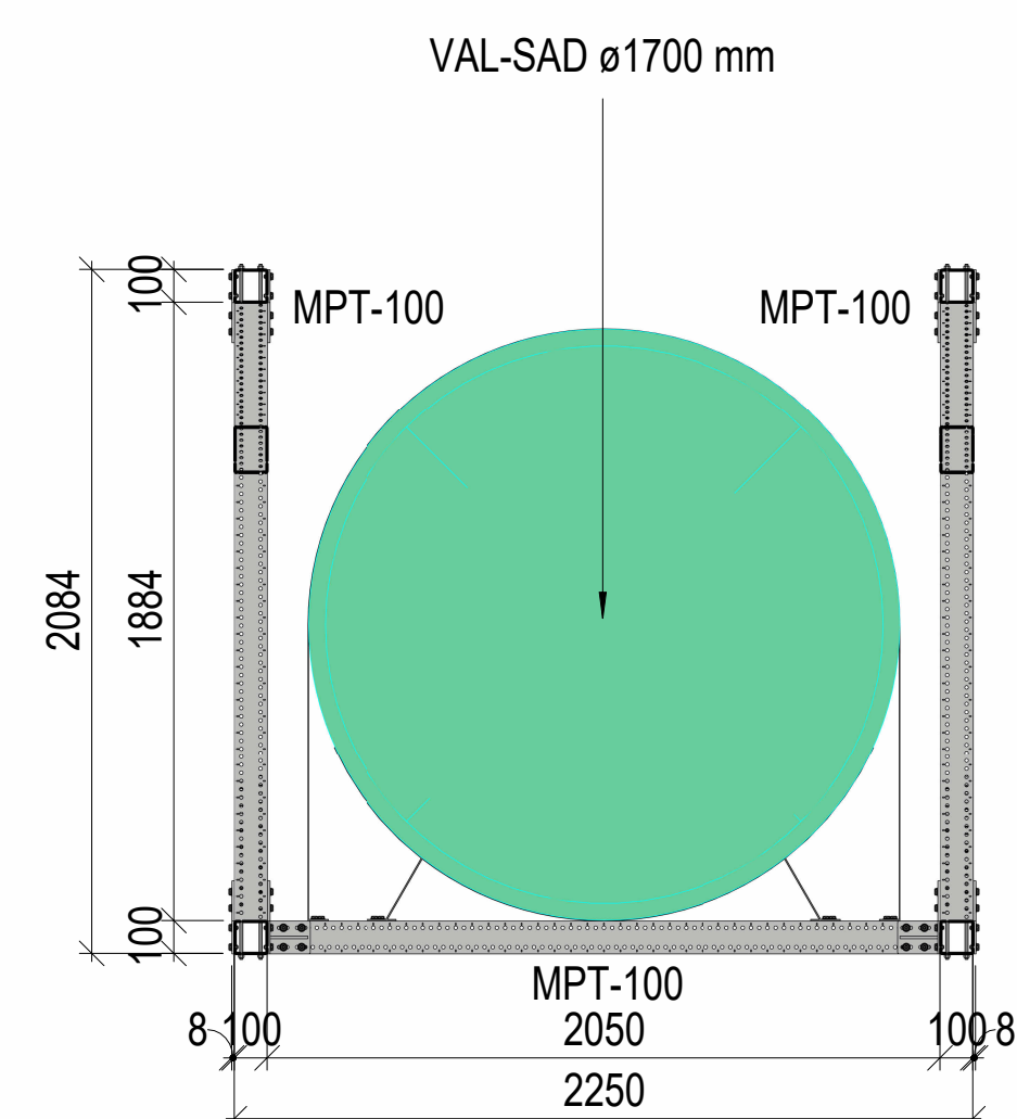
SECTION A
