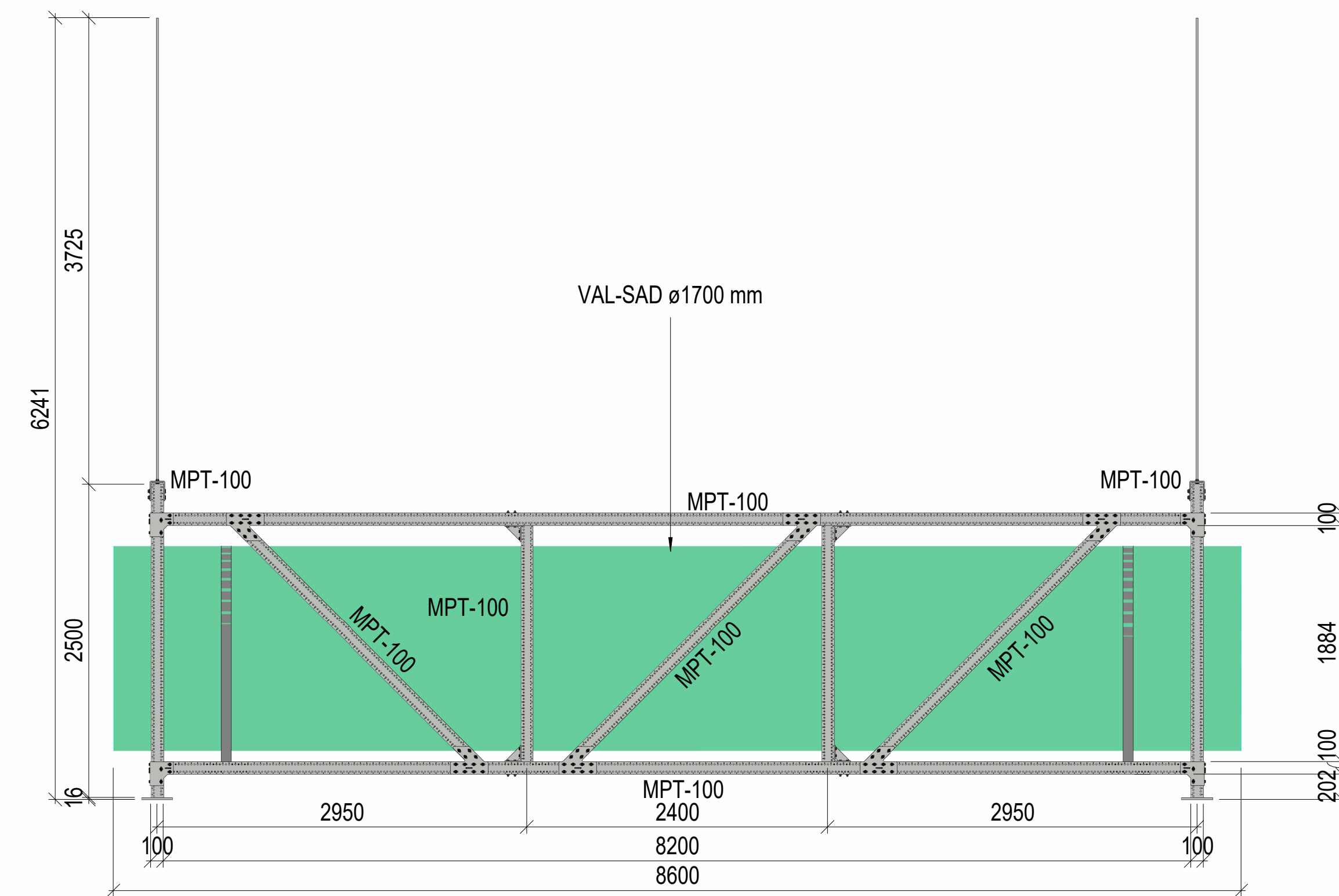
SECTION F
