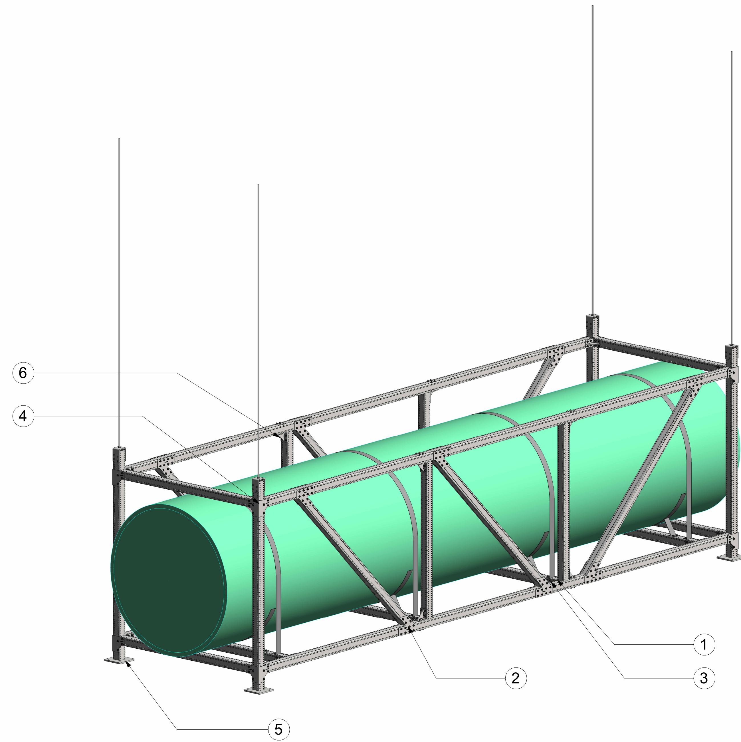
3D VIEW
