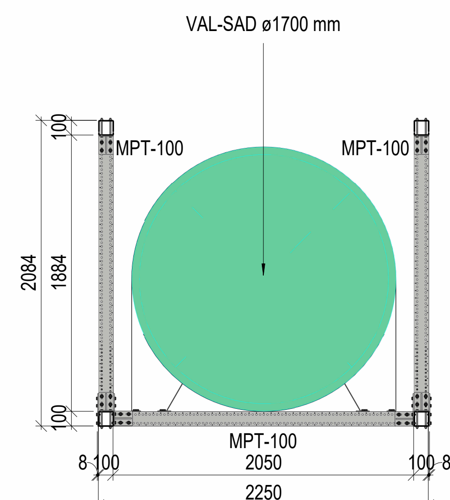
SECTION B
