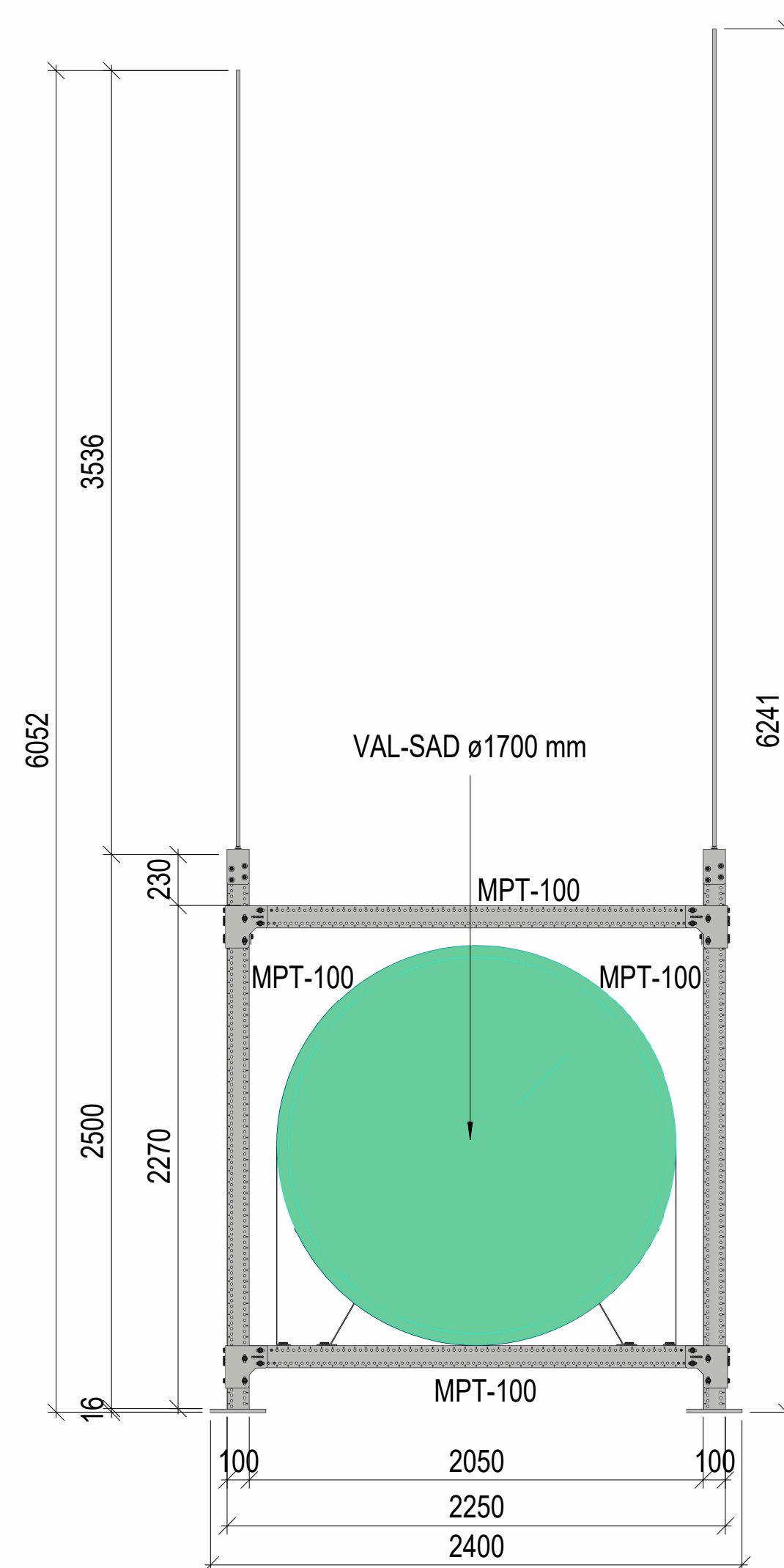
SECTION D
