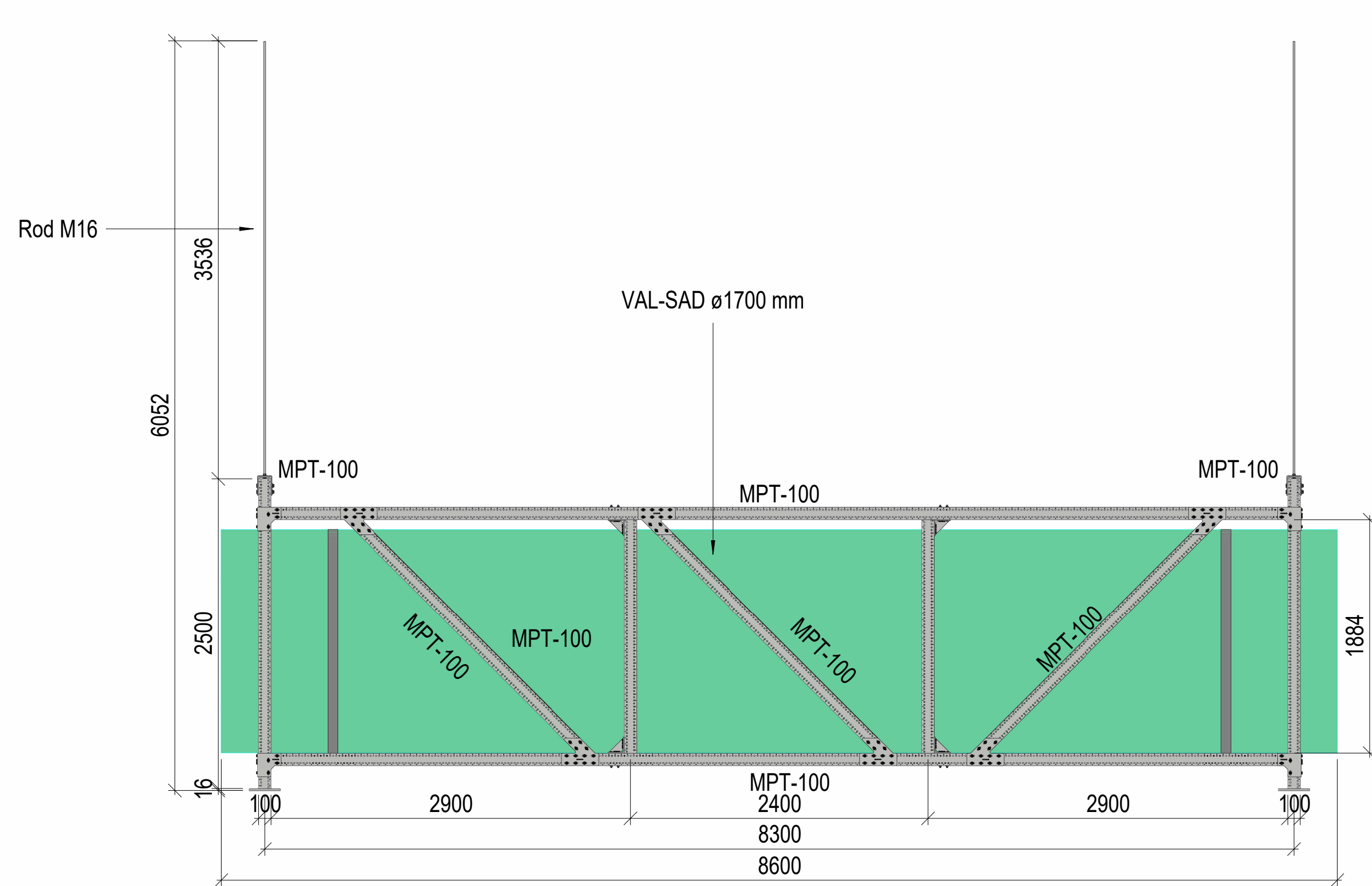
SECTION E
